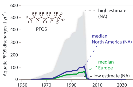
Figure 1. Direct continental inputs of PFOS to the North Atlantic Ocean (20° N–60°N) from European and North American (U.S. and Canada) wastewater and rivers between 1958 and 2010. Median estimates are shown as the solid line and shaded grey indicates 95% confidence intervals for North American releases. European inputs are based on Pistocchi and Loos [2009].
