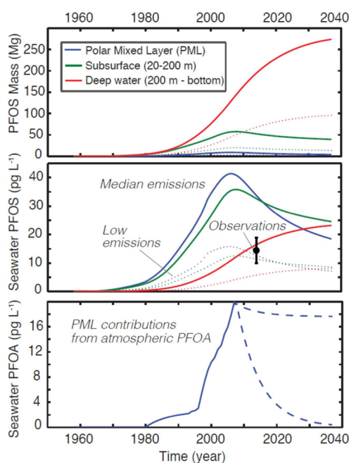
Figure 5. Modeled PFOS and PFOA concentrations in surface waters (PML, 0–20 m), subsurface (including the halocline, 20–200 m), and deep waters (200 m–bottom) of the Arctic Ocean based on the geochemical box model adapted from Soerensen et al. 38 For PFOS, median and low emissions scenarios represent uncertainty in the magnitude of historic discharges from North American and European wastewater and rivers into the North Atlantic Ocean, that then circulate into the Arctic based on the 3-D ocean simulation of Zhang et al. 39 For PFOA, resolved oceanic inputs are not available, thus we used deposition rates from the Devon ice cap in the Canadian High Arctic to estimate the contribution of atmospheric inputs to those observed in the polar mixed layer (PML) in this work (bottom panel). Dashed lines represent alternate assumptions for deposition after 2007: the top line assumes deposition values from 2007 continue, and the bottom line assumes zero deposition.
