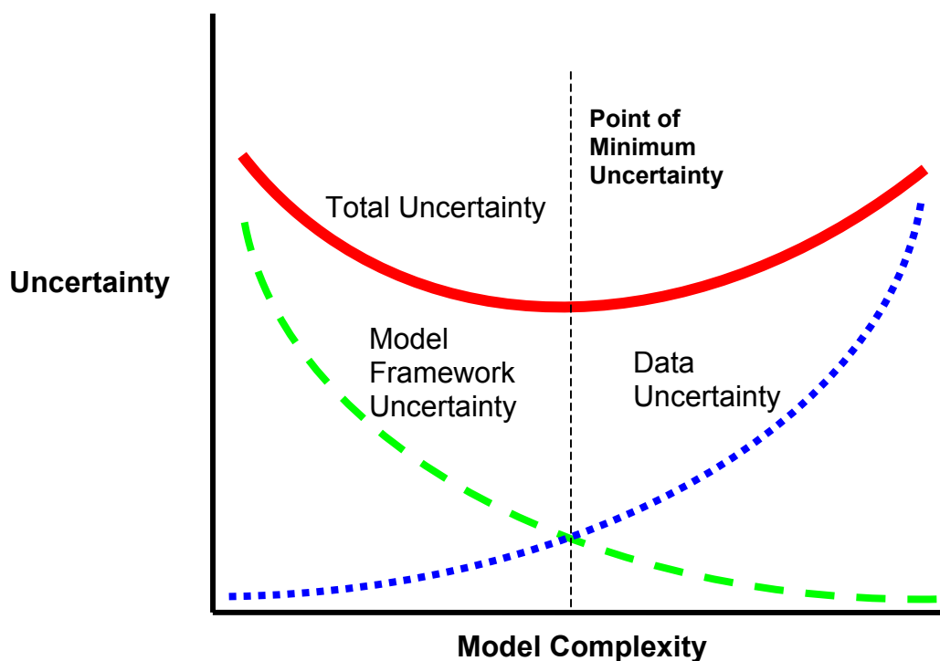
Figure 2. Illustration of relationship between model framework uncertainty and data uncertainty, and the combined effect on total model uncertainty. In this guidance, uncertainty is the term used to describe incomplete knowledge about specific factors, parameters (inputs) or models. Model framework uncertainty is a function of the soundness of the underlying scientific foundations of the model. Data uncertainty measurement errors, analytical imprecision and limited sample sizes during the collection and treatment of data that are used to characterize model parameters. An optimal level of complexity exists for every model, which is represented in the figure as the “point of minimum uncertainty.” (Adapted from Hanna [11]).
